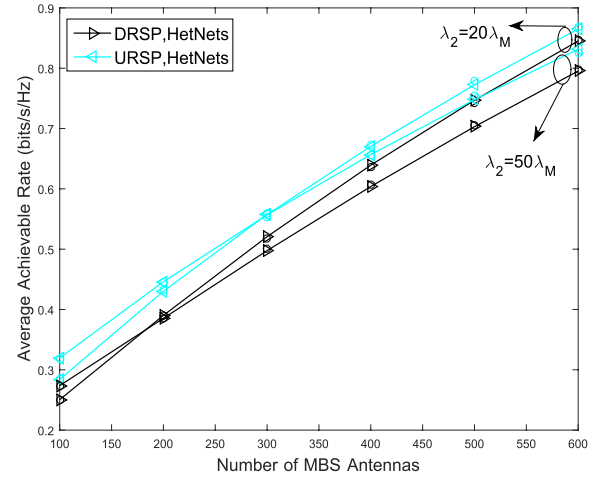
Fig. 10. The average uplink achievable rate against the number of antennas in the massive MIMO HetNet.
