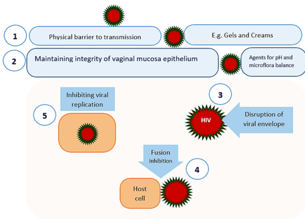
Figure 5: Potential target sites and mode of action for microbicides in preventing HIV transmission.
