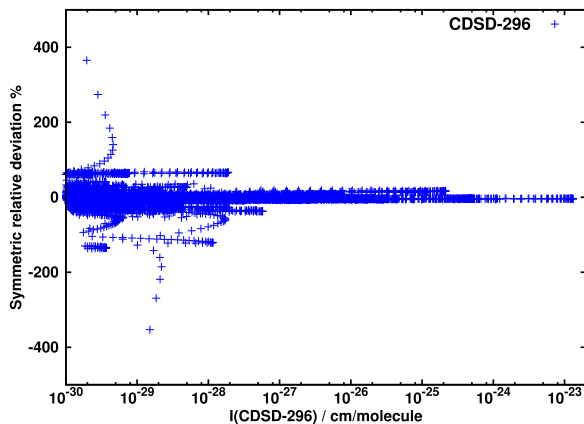
Fig. 16. Symmetric relative intensities (cf. Eq. (2)) plotted against CDS-296 line intensities for the 828 isotopologue. Only the \pm 500\% region is depicted.
