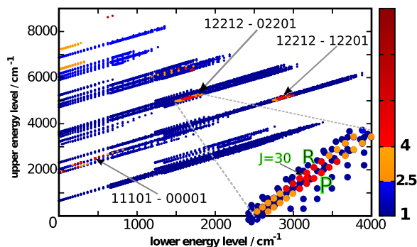
Fig. 2. Scatter factor map for the 828 isotopologue. Color coding denotes respective classification of lines: blue stands for stable lines, orange for intermediate lines and red for unstable lines. The arrows indicate selected bands for which a J -localized peak in the scatter factor is observed. The zoomed inset in right bottom corner shows the peak region of the scatter factor for the 12212–02201 band. Both P and R branches are affected by the interaction around J=30 . (For interpretation of the references to color in this figure caption, the reader is referred to the web version of this paper.)
