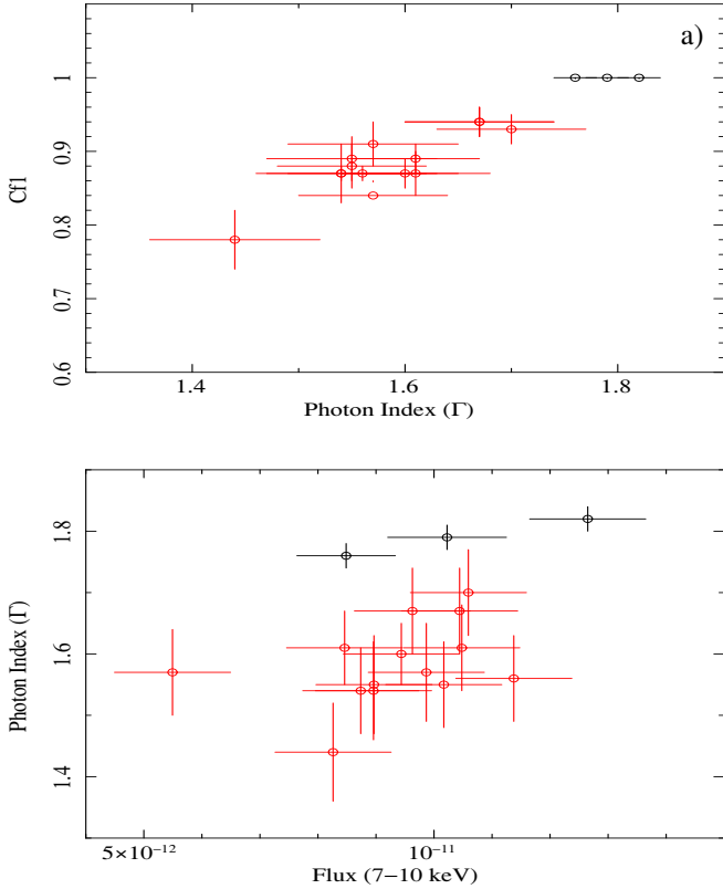
Fig. 10. (Panel a ) Spectral fit parameters \Gamma versus C_{f_1} (panel a ) and (panel b ) \Gamma versus power law F_{7-10\text{ keV}} (panel b ). Archival observations are indicated in black, while those from the campaign are indicated in red.
