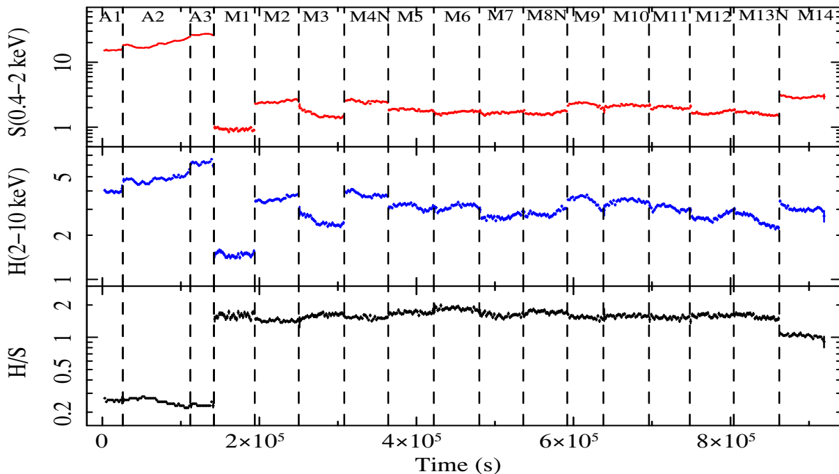
Fig. 1. Background subtracted XMM-Newton pn light curves of NGC 5548 calculated for the soft (S) 0.4–2 keV energy band (top), the hard (H) 2–10 keV energy band (middle) and their hardness ratios H/S (bottom). Vertical dashed lines indicate when observations were interrupted during the years.
