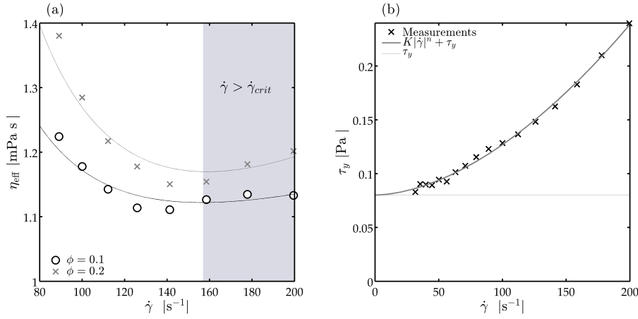
Fig. 10 Variation in the effective viscosity of Chlorella sp. suspensions at high shear rates (a) for two cell concentrations. The shaded region ( \dot{\gamma} > 156 s -1 ) corresponds to the region where the effective viscosity is predicted to increase with strain rate, according to the Herschel-Bulkley model (Equation 5). The variation in the stress with strain rate for the \phi = 0.2 case is shown in (b), along with the estimated flow curves (Equation 4) and the contribution of the yield stress. The trend of increasing stress with strain rate (i.e. the shear-thickening behaviour) is particularly clear here.
