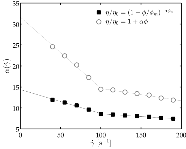
Fig. 6 Variation in the intrinsic viscosity estimated using the Einstein and Krieger-Dougherty equations with strain rate, for T. chuii suspensions.
