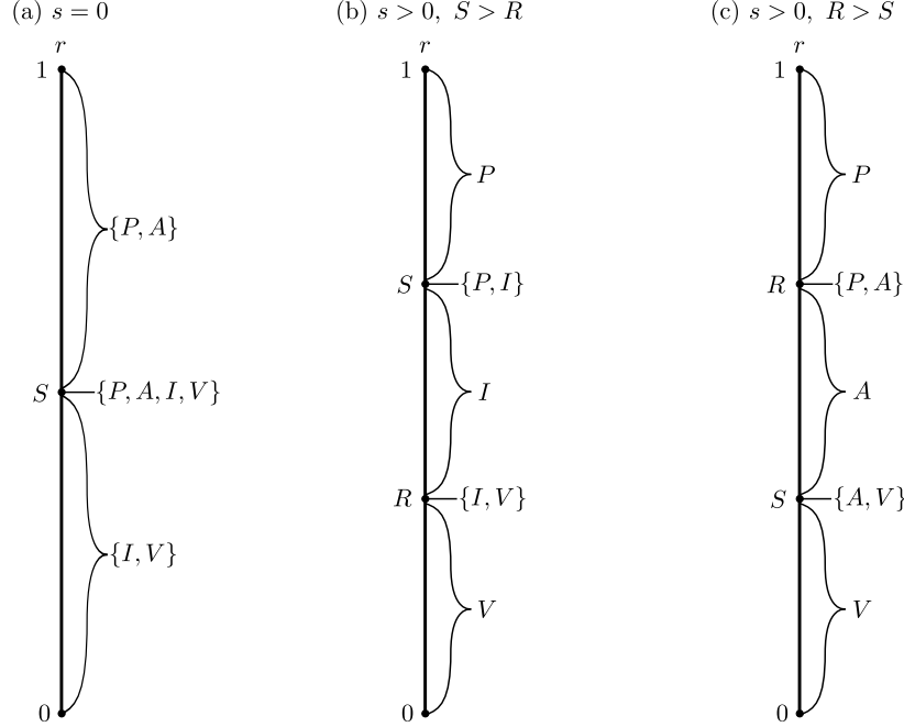
Figure 1: A graphical representation of the best response function BR_i(s, r) under the three cases: (a) s = 0 , (b) s > 0, S > R , and (c) s > 0, R > S .
