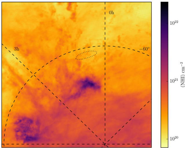
Figure 7. H I gas column density map from Kalberla & Haud (2015), in zenithal equal area projection, close to the south celestial pole. A grid of equatorial coordinates ( \alpha and \delta ) is indicated. The SMC is close to the centre of the figure and the LMC is located near the bright spot in the lower-left corner. No significant excess of H I gas is observed at the position of the SMCNOD (dotted ellipse).
