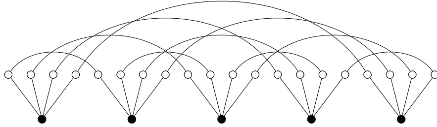
(a) First subdivide each edge to isolate each of the high degree vertices.
