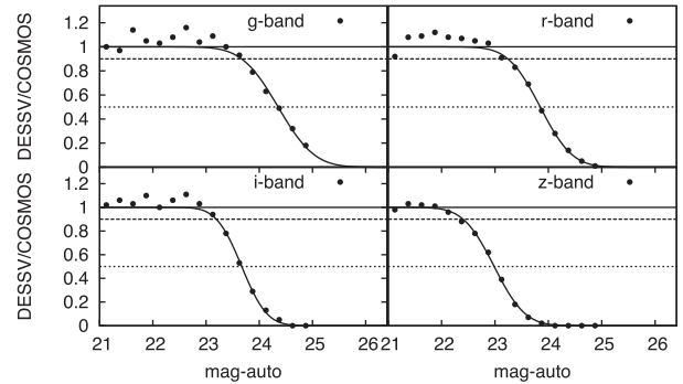
Figure 2. Completeness functions in each band for SPT-CL J0423-6143. We compare the object counts observed towards the cluster to the counts from deeper data from the COSMOS survey. The resulting completeness curve is fit by an error function, which we use to estimate 50 per cent and 90 per cent completeness.
