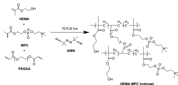
Fig. 1. Synthesis of HEMA-MPC hydrogel films by free radical polymerisation. The two monomers (HEMA and MPC) were mixed with the crosslinker (PEGDA) to form a clear solution. AIBN (initiator) was added and placed in the oven at 70°C for 6 hours.
