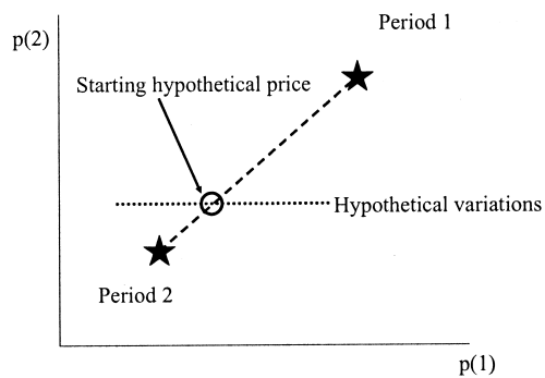
FIGURE 12. Convex combination.
