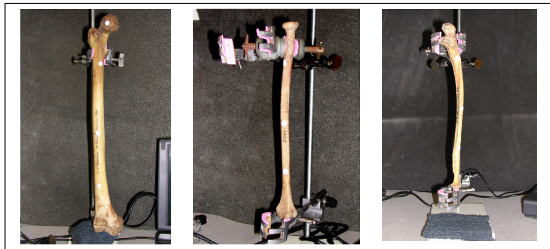
Figure 3-1 Specimen set up for the femur, radius and ulna using clamps and a test tube stand.
