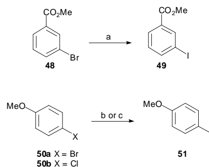
Scheme 10 a. KI (2.5 eq), cat. \text{NiBr}_2 , Zn, HMPA, 50 °C, 81%. b. Ni (s), KI (2 eq), DMF, 150 °C, 76% (X=Br). c. Ni (s), NaI (5 eq), DMF, 150 °C, 55% (X=Cl).
