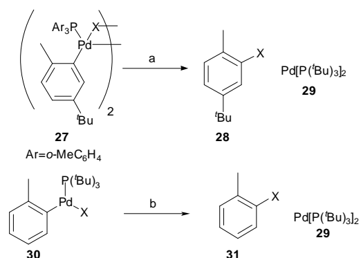
Scheme 4 a. \text{P}(\text{tBu})_3 (15 eq), \text{C}_6\text{D}_6 , 70^\circ\text{C} , 70% (X=Cl, Br), 39% (X=I); b. \text{P}(\text{tBu})_3 (20 eq), \text{C}_6\text{D}_6 , 70^\circ\text{C} , 76% (X=Cl), 98% (X=Br), 79% (X=I).
