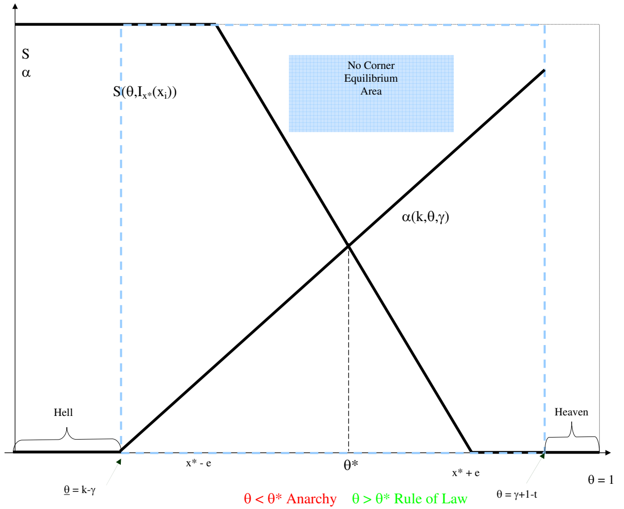
Figure 7: Equilibrium: \theta^*
