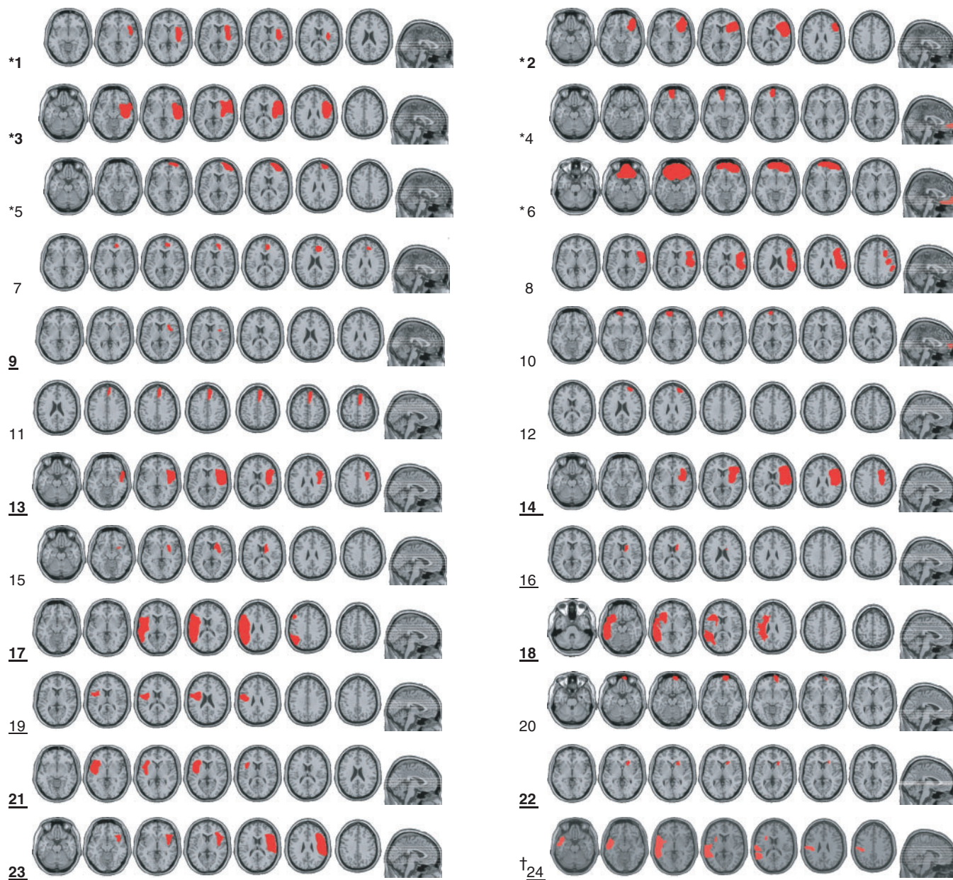
Fig. 2 Lesion regions of interest displayed on a transverse view of a standard T1 MRI template image. Bold numerals indicate patients who were impaired at the rule switching task. Underscored numerals indicate impairment in antisaccade task. †No data available for rule switching. *No data available for antisaccades.
