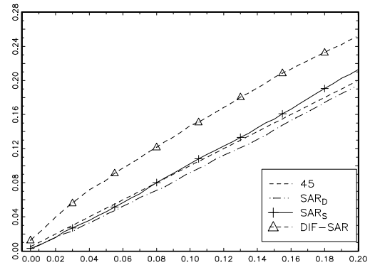
Figure 12. \rho = 0.95, \alpha = 0.95, T = 4
