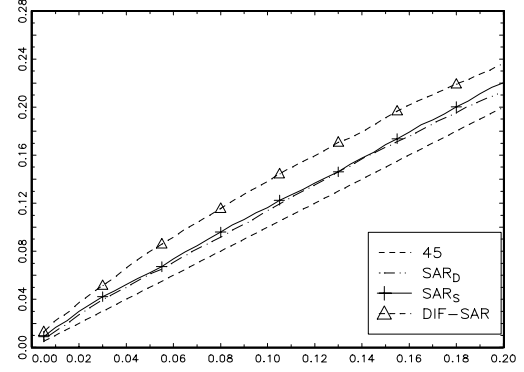
Figure 4. p-value plot, \rho = 0.95 , T = 4
