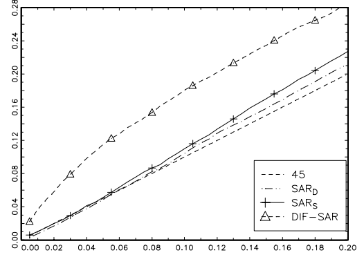
Figure 10. \rho = 0.5, \alpha = 0.95, T = 8
