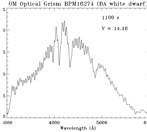
Fig. 4. Spectrum of the white dwarf BPM16274 obtained using the visual grism. The regular low-level fluctuations in the signal with wavelength are due to the modulo-8 pattern (section 5.6.3), which has not been corrected in this plot.
