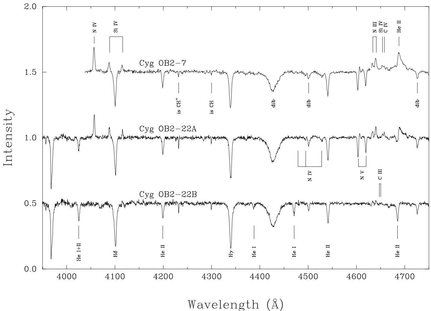
FIG. 1.—Rectified linear-intensity, blue-violet spectrograms of the spatially resolved components of Cyg OB2-22 , with Cyg OB2-7 for comparison. The stellar features identified above the spectrum of No. 7 are N IV \lambda 4058 ; Si IV \lambda\lambda 4089-4116, 4654 ; N III \lambda\lambda 4634-4640-4642 ; C IV \lambda 4658 ; and He II \lambda 4686 ; the wavelengths of the interstellar lines and diffuse interstellar bands identified below are given by Walborn & Howarth (2000). The lines identified in Cyg OB2-22A are N IV \lambda\lambda 4478-4496-4530 and N V \lambda\lambda 4604-4620 ; in Cyg OB2-22B they are He I \lambda\lambda 4026 (+II), 4387, 4471 ; H \delta \lambda 4102 ; H \gamma \lambda 4340 ; He II \lambda\lambda 4200, 4541, 4686 ; and (above) the C III \lambda 4650 blend.
