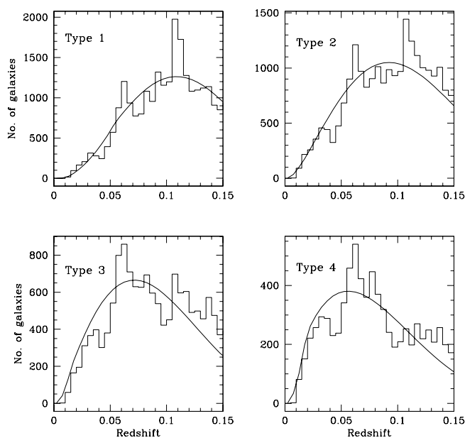
Figure 13. Comparison between the observed N(z) distributions (histograms) and the predicted N(z) for each spectral type ( b_J < 19.3 ). Note that the N(z) distributions of the first two types are recovered very well but that significant deviations exist for the last two (most active star-forming) types.
