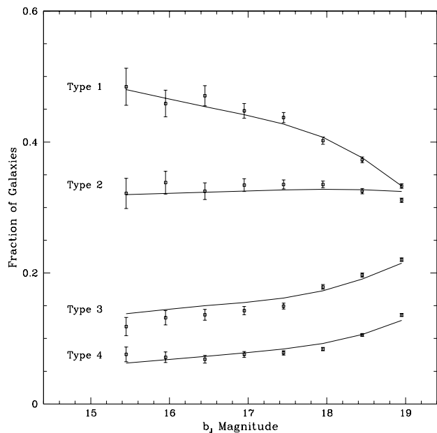
Figure 12. A test recently proposed by Kochanek, Pahre & Falco (2000). We show observed (squares) and predicted (lines) type fractions for the 2dF galaxies used in our calculations, where the predicted fractions have been derived from integrating our LFs. The two are consistent within the stated (Poisson) errors.
