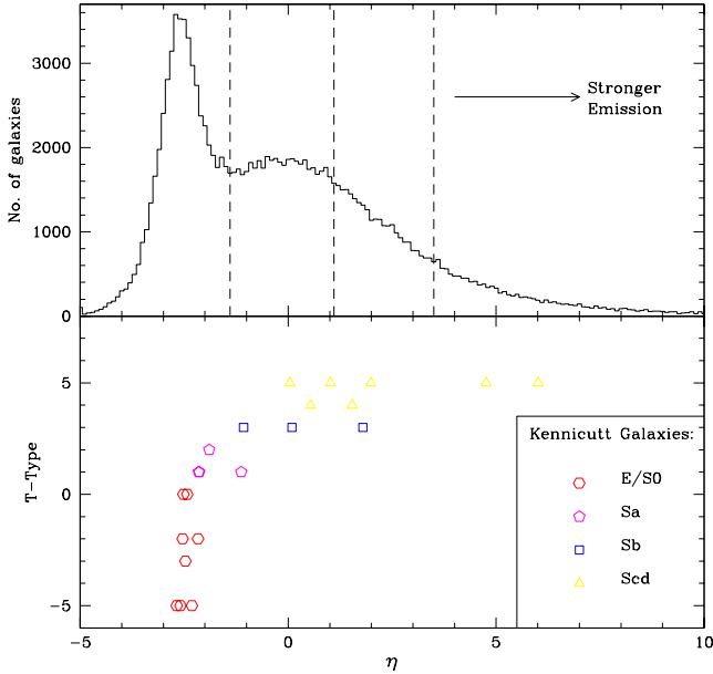
Figure 4. The observed distribution of spectral type measured by \eta . Also shown are the four divisions we use to divide the dataset (see Fig. 7 for mean spectra). The bottom panel shows the correlation between \eta and morphological type using a training set of galaxies taken from the Kennicutt Atlas (Kennicutt 1992).
