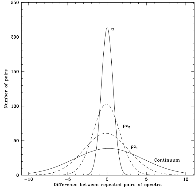
Figure 5. Dispersion in the PCA projections ( pc_1 and pc_2 ) and in the spectral classification \eta . These distributions are well fit by Gaussians (shown here) and were calculated by taking the differences in these quantities between \sim 2000 repeated spectral observations. Also shown is the dispersion in the orthogonal projection to \eta , which quantifies the continuum slope in the spectra.
