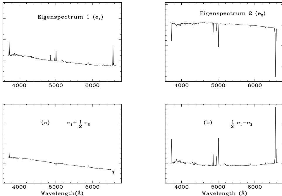
Figure 3. The first two eigenspectra are shown in the top two panels and the linear combinations which either minimise (a) or maximise (b) the effect of emission/absorption features are shown in the bottom two.
