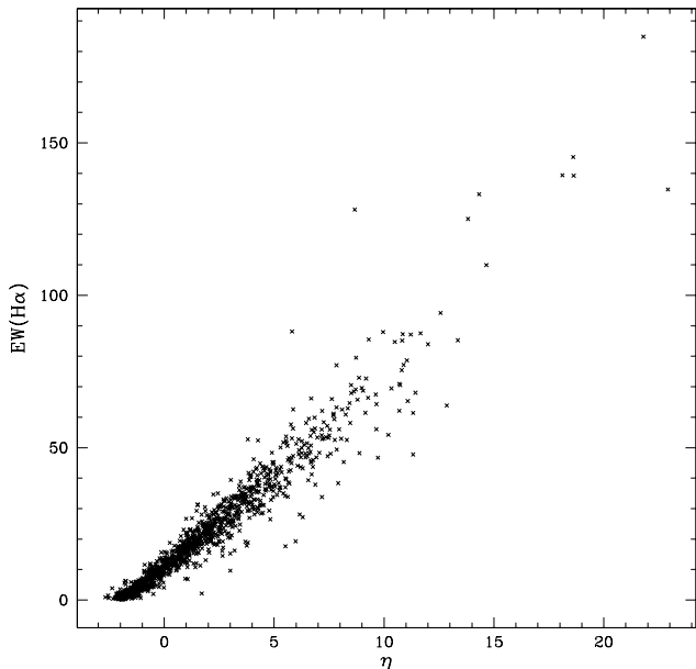
Figure 6. The EW(H\alpha) is very tightly correlated to \eta for emission line galaxies (see Bland-Hawthorn et al., in preparation, for further details).
